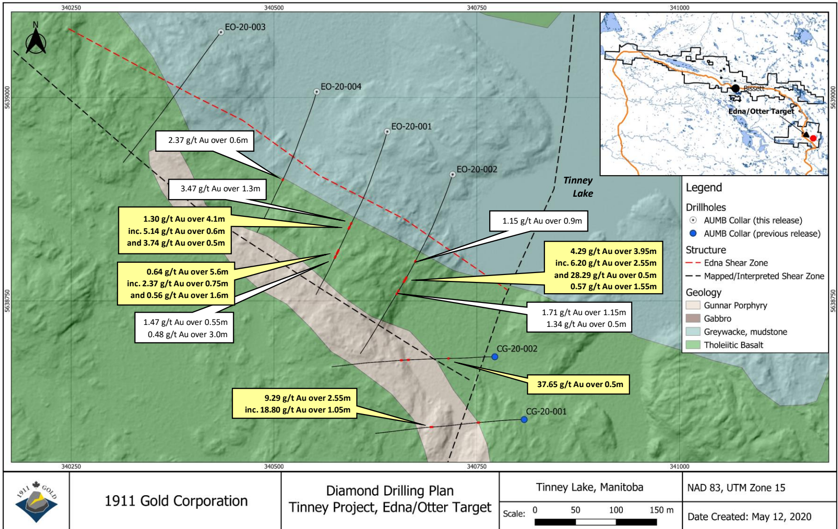
Figure 3: Plan map of the Edna-Otter (EO) target, showing drillhole locations and major structures. Map base is a shaded-relief LiDAR DEM with bedrock geology drape. Drillhole intercepts of less than 1 g/t Au over less than 1.0 m are omitted for clarity (refer to Table 1 for complete listing).
