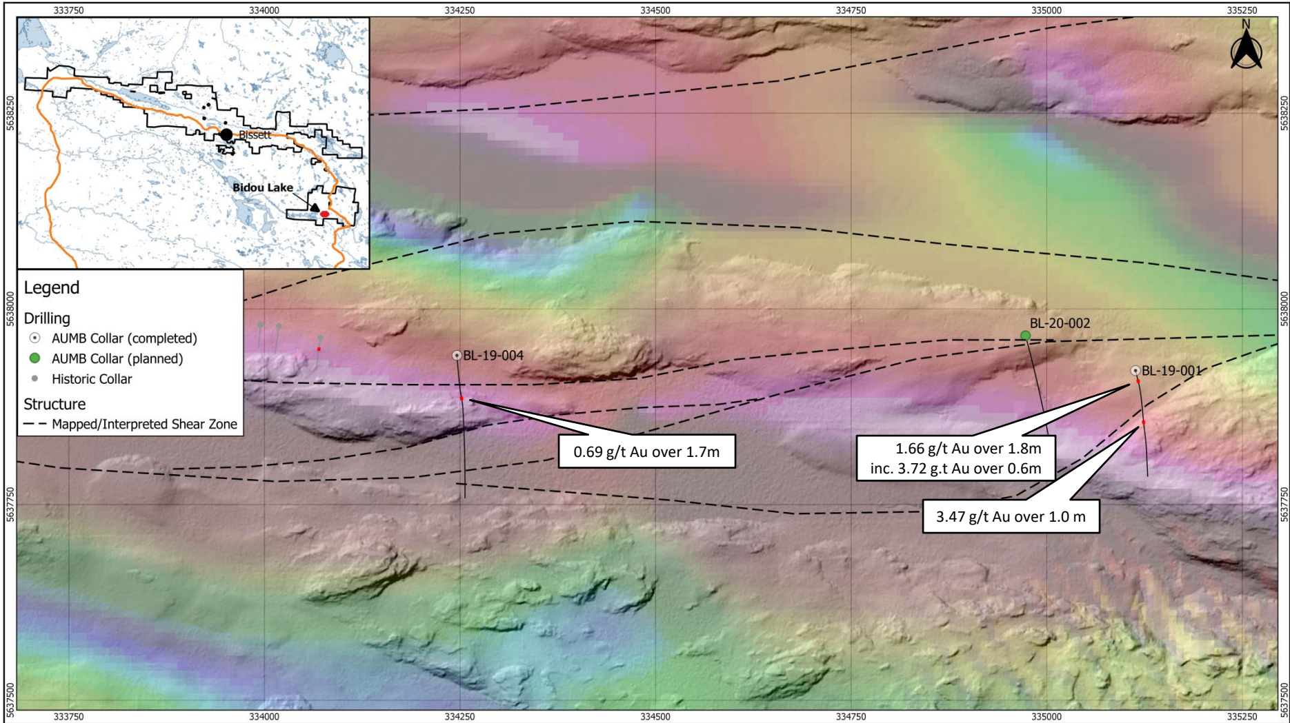
Plan map of the Bidou South Target, showing drillhole locations and major shear Zones. Map base is a shaded-relief LiDAR DEM with AMAG (TMI-Tilt) drape.
