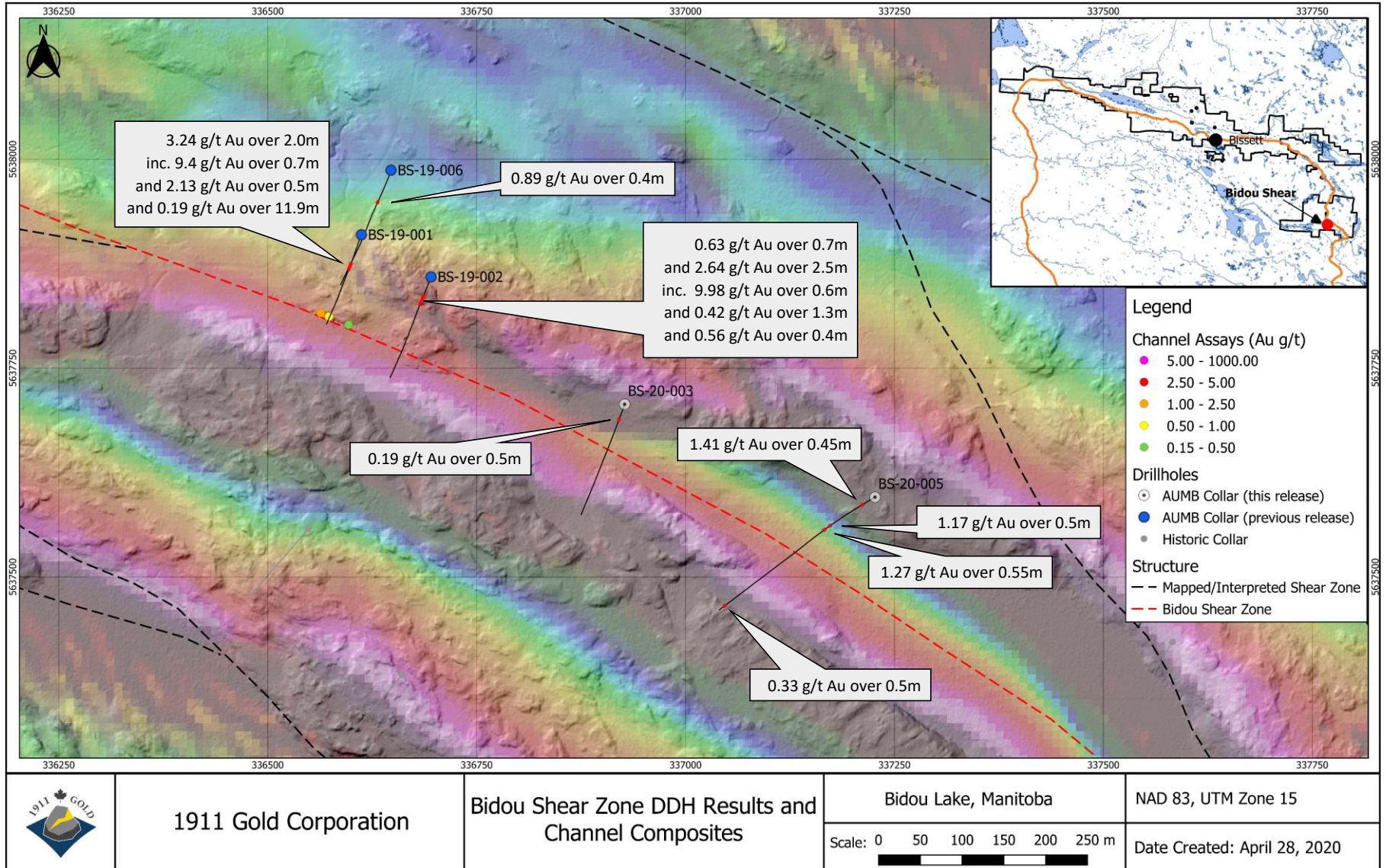
Figure 3: Plan map of the Bidou Shear Target, showing channel sample and drillhole locations, and major shear zones. Map base is a shaded-relief LiDAR DEM with AMAG (TMI-Tilt) drape.
