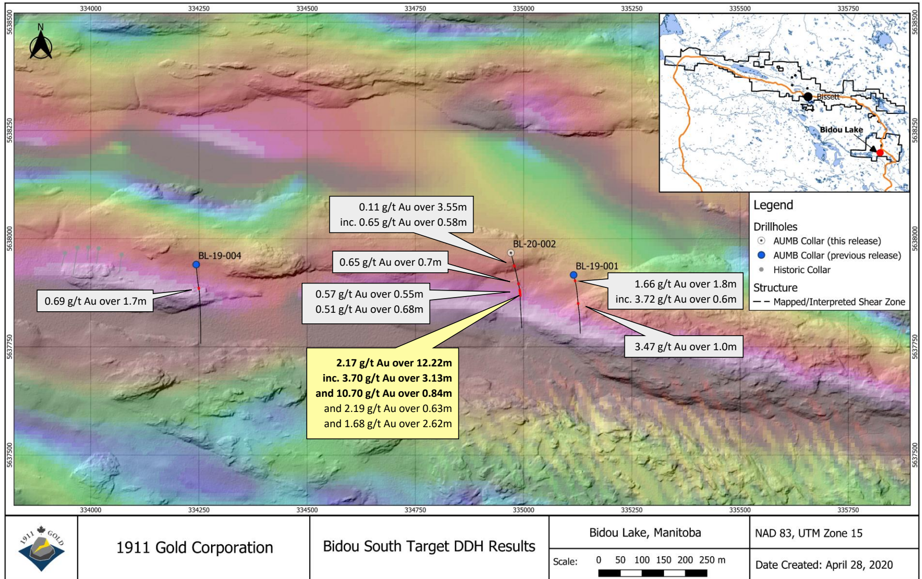
Figure 4: Plan map of the Bidou South Target, showing drillhole locations and major shear Zones. Map base is a shaded-relief LiDAR DEM with AMAG (TMI-Tilt) drape.
